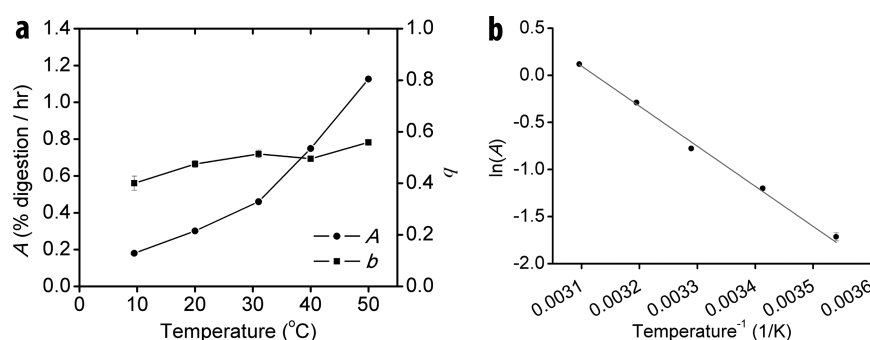
Figure 2. Dependence of A and b on temperature. (a) Experimentally determined A and b values for the TfCel9A digestion of BC at different temperatures and (b) Arrhenius plot of A . A time-course profile was obtained for each temperature ( N = 3), and the data were fit with eq 6 to obtain the A and b values. Error bars represent the standard error of the fit.
