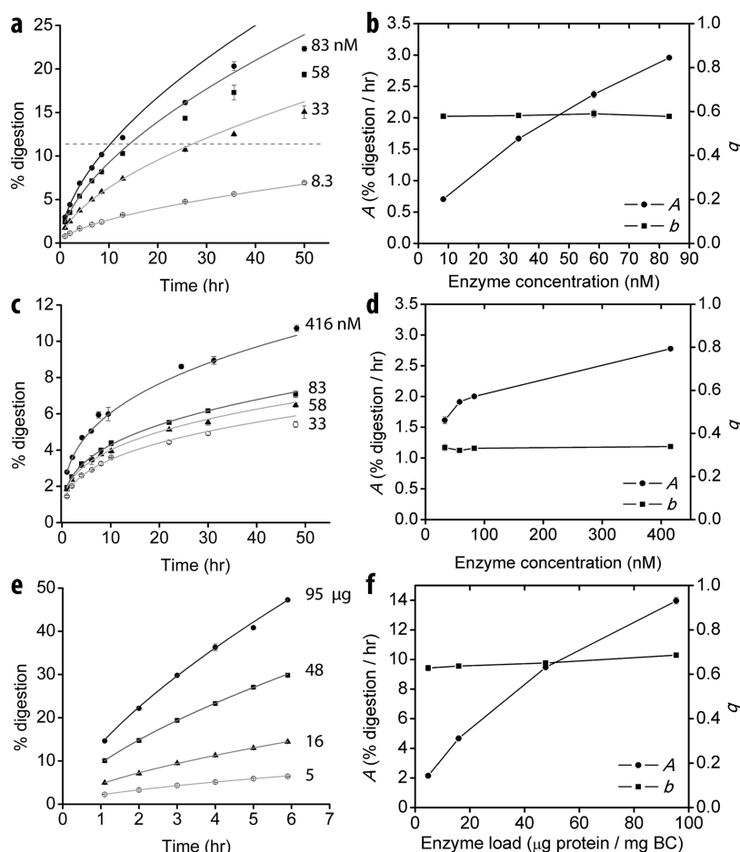
Figure 3. Dependence of A and b on enzyme concentration. Different concentrations of TfCel9A (a, b) TfCel5A (c, d), and T. fusca crude supernatant (e, f) on BC. All time-course data were obtained in triplicate. The error bars in panels a, c, and e represent standard deviation. The time-course data were fit with eq 6, and the obtained A and b values are plotted in panels b, d, and f; the error bars represent standard error. The dashed line in panel b indicates the approximate drop-off value (above which the digestion rate decreases more rapidly than predicted by the initial fit).
