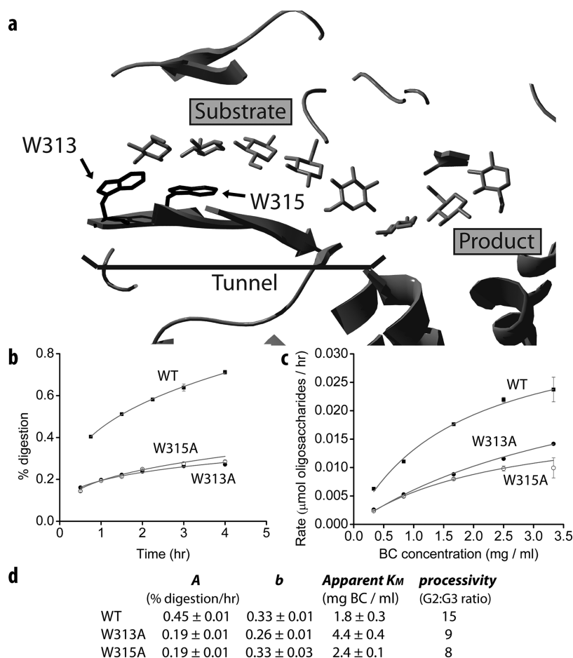
Figure 5. Role of W313 and W315 in the digestion of BC by TfCel48A. (a) Tunnel and active site of TfCel48A. The W313 and W315 residues are located at the mouth and inside the tunnel, respectively; (b) time-course profiles of WT, W313A, and W315A on BC ( N = 3 ) fitted with eq 6; (c) apparent K_M experiments with WT, W313A, and W315A on BC; and (d) eq 6 parameter values, processivity, and apparent K_M of WT and mutated TfCel48A. Processivity is calculated as the ratio of cellobiose (G2) to cellotriose (G3). 33
