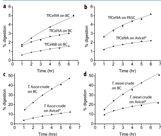
Figure 1. Fitted digestion curves for different enzymes on various substrates. (a) T. fusca Cel9A, Cel5A, and Cel6B on BC (33.3 nM each enzyme); (b) T. fusca Cel9A on Avicel (167 nM enzyme) and phosphoric acid-swollen cellulose (PASC; 33.3 nM enzyme); (c) T. fusca crude supernatant on BC (95 \mu g total protein/mg substrate) and Avicel (159 \mu g total protein/mg substrate); and (d) T. reesei crude supernatant on BC (8 \mu g total protein/mg substrate) and Avicel (80 \mu g total protein/mg substrate).
