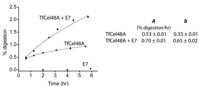
Figure 4. Effect of the auxiliary protein T. fusca E7 (AA10) on the digestion of BC by weak T. fusca exocellulase TfCel48A. Time-course data were collected in triplicate and were fit to eq 6. The calculated parameters are presented in the table inset. E7 alone produces only trace amounts of soluble sugars, and its time course profile does not follow eq 6.
